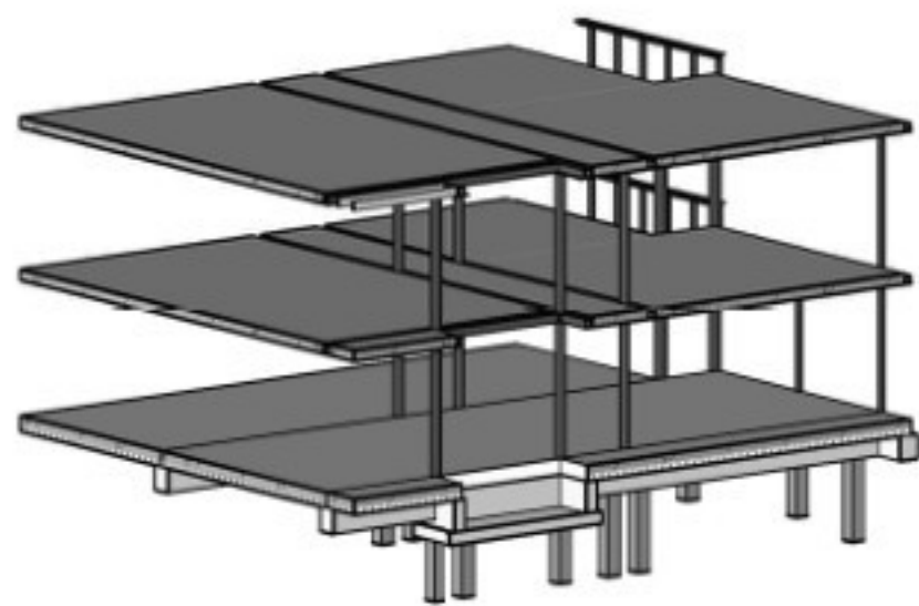
3D ISOMETRIE (FRAGMENT LIFTPUT)
